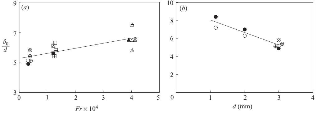
FIGURE 3. Dependence of dimensionless flowing layer thickness on (a) Froude number for 3 mm steel beads and (b) bead size for Fr = 0.39 \times 10^{-4} . Symbols: \bullet , Fr = 0.39 \times 10^{-4} ; \blacksquare , Fr = 1.26 \times 10^{-4} ; \blacktriangle , Fr = 4.03 \times 10^{-4} . Symbol fill: open, air; black, water; open with a ‘+’ in the middle, 38% glycerine; open with a ‘x’ in the middle, 56% glycerine; and open with a horizontal line, 63% glycerine. In some cases, data points that would overlay one another are shifted horizontally by a small amount to make all data points visible.
